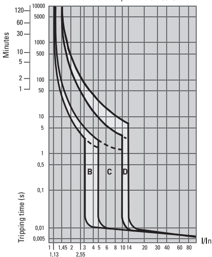
Figure 1. Tripping curves
